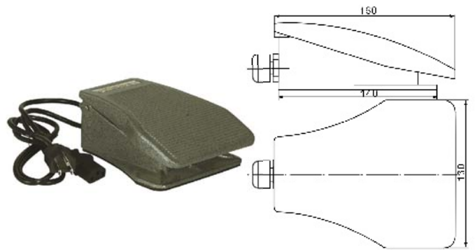
LLJFS12 (调速式Speed governing type)
